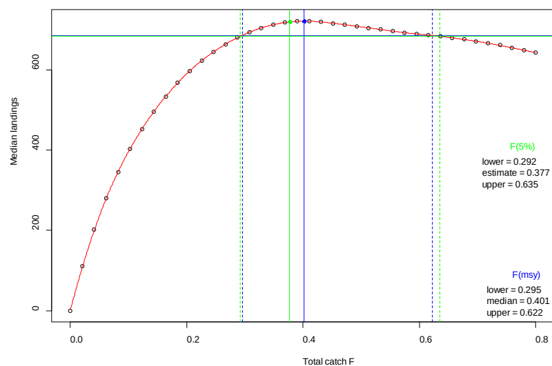
Figure 6.14.4. Sole IIIa based on full S-R timeseries, with fixed F exploitation from F = 0 to 0.8. Median landings yield curve with estimated reference points. Blue lines: F_{MSY} estimate (solid) and range at 95% of maximum yield (dotted). Green lines: F(5\%) estimate (solid) and range at 95% of yield implied by F(5\%) (dotted).
