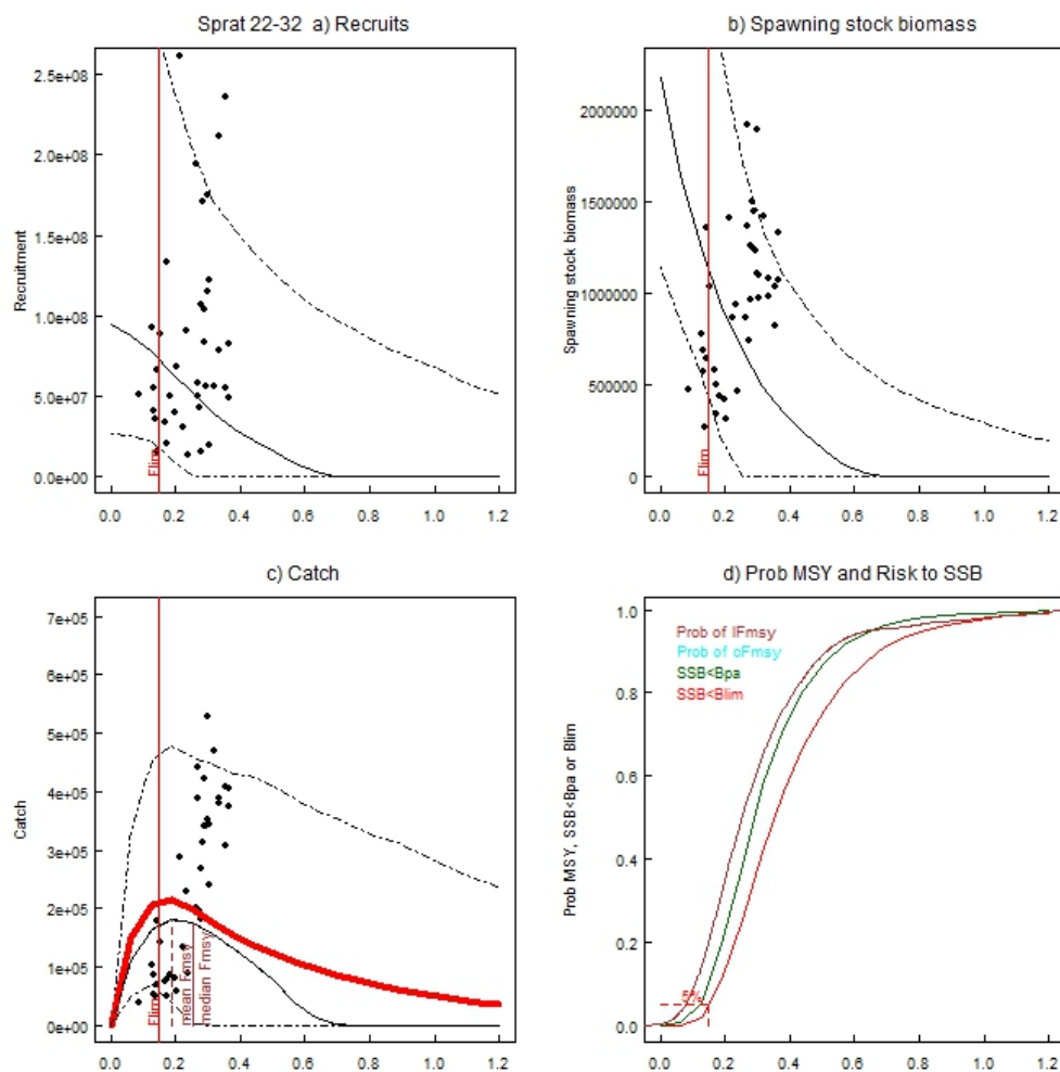
Figure 6.13.3. Eqsim results applying the standard regression method for Sprat in Subdivisions 22–32 without B_{\text{trigger}} . Panels a-c: historic values (dots) median (solid black) and 90% intervals (dotted black) recruitment, SSB and landings for exploitation at fixed values of F . Panel c also shows mean landings (red solid line). Panel d shows the probability of SSB < B_{\text{lim}} (red), SSB < B_{\text{pa}} (green) and the cumulative distribution of F_{\text{MSY}} based on yield as landings (brown) and catch (cyan).
